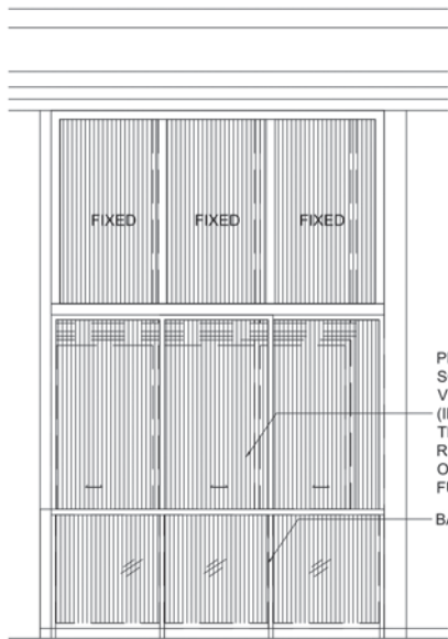
#44-01, #44-02, #44-04, #44-06, #44-08, #44-09, #44-10, #44-11, #44-12: TYPICAL RETRACTABLE BALCONY SCREEN (CLOSED) - ELEVATION 1
