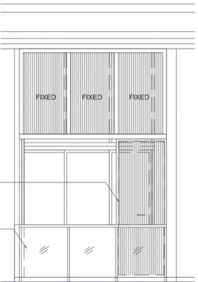
#44-01, #44-02, #44-04, #44-06, #44-08, #44-09, #44-10, #44-11, #44-12: TYPICAL RETRACTABLE BALCONY SCREEN (OPEN) - ELEVATION 2
