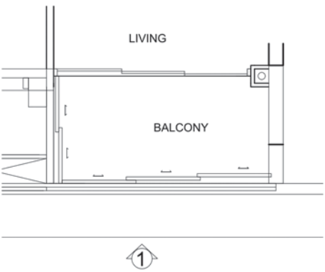
#44-01, #44-02, #44-04, #44-06, #44-08, #44-09, #44-10, #44-11, #44-12: TYPICAL RETRACTABLE BALCONY SCREEN (CLOSED) - PLAN
